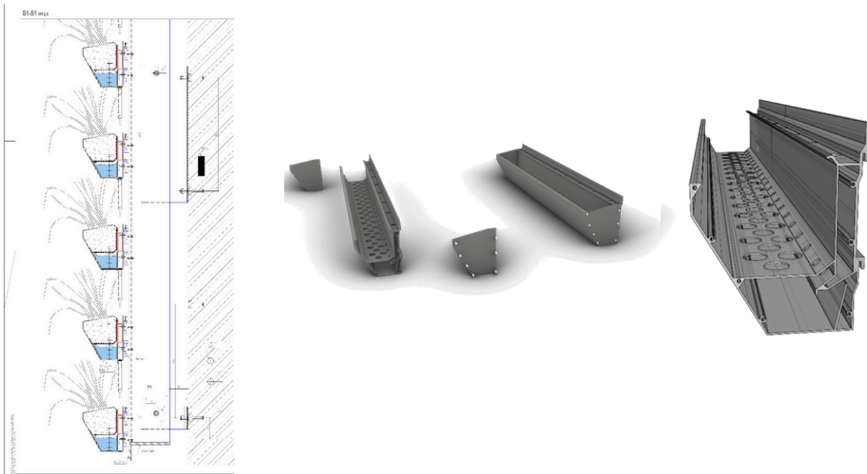
Figure 83: Design of the prototype planter, drawn for the installation in Aachen
