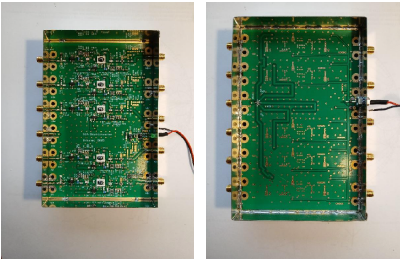
Figure 129: Assembled 5-channel downconverter board for 3.5 GHz band – top (left) and bottom (right).
