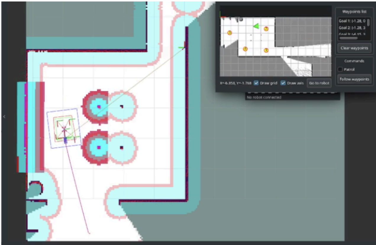
Figure 192: Example of navigation controlling via AmurCore
