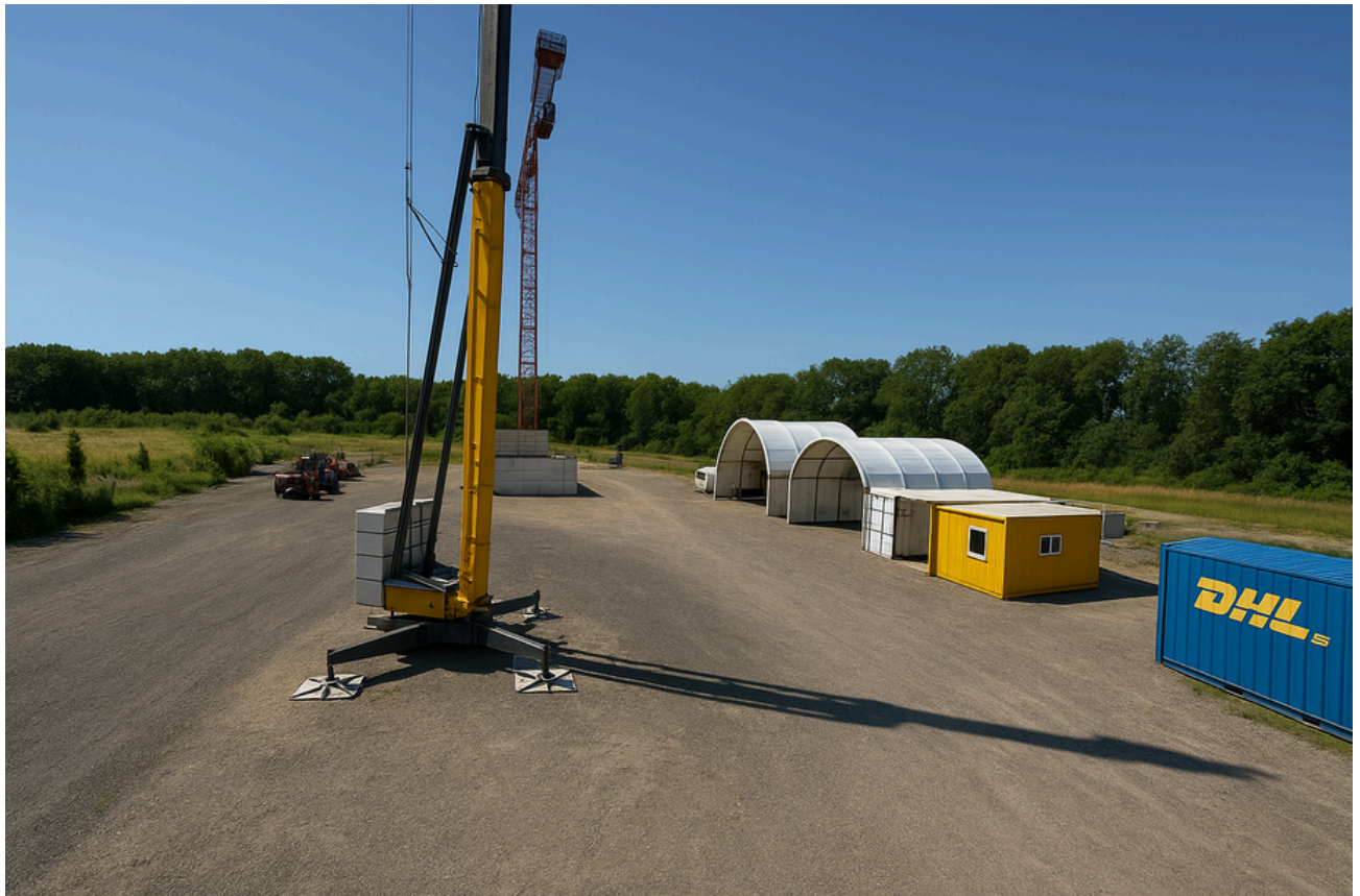
Figure 46: Testing 5G solution at Aachen (showing locations of anchors and anchor ID's).
