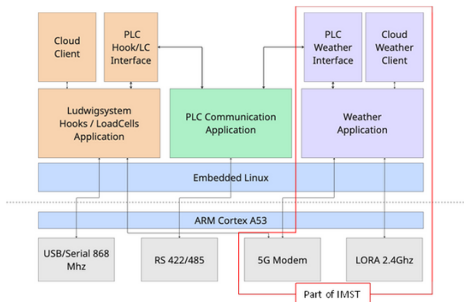
Figure 102: Software architecture of the IoT-Gateway
