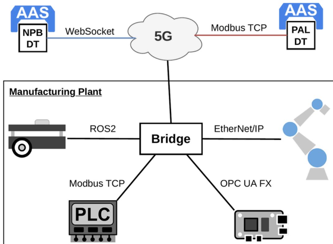
Figure 122: Production Assembly Line use case.
