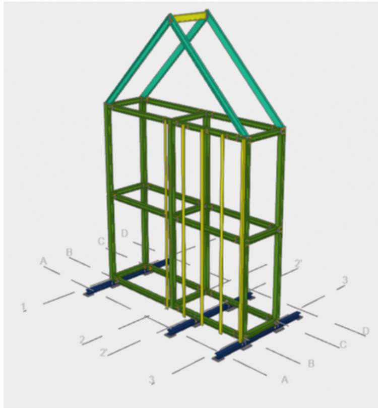
Figure 120: Steel Construction
