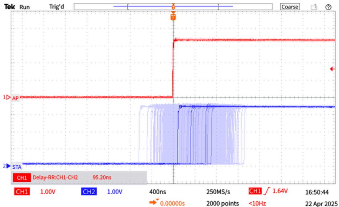
Figure 166: Clock-synchronization performance over the air.
