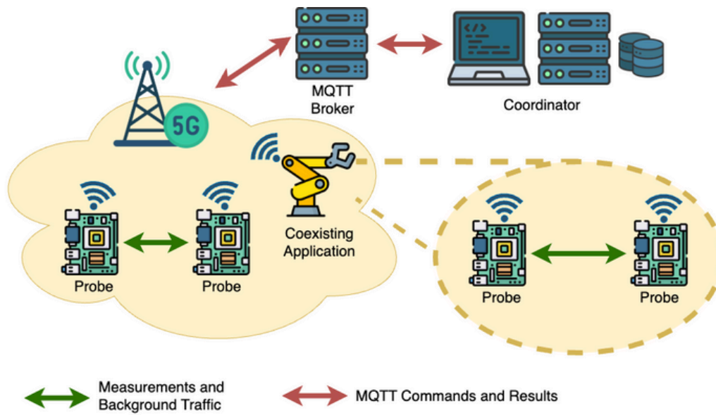
Figure 84: Measure-X architecture.
