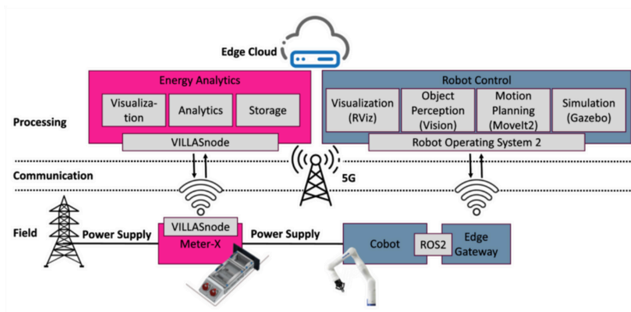
Figure 30: Architectural goal of the project.
