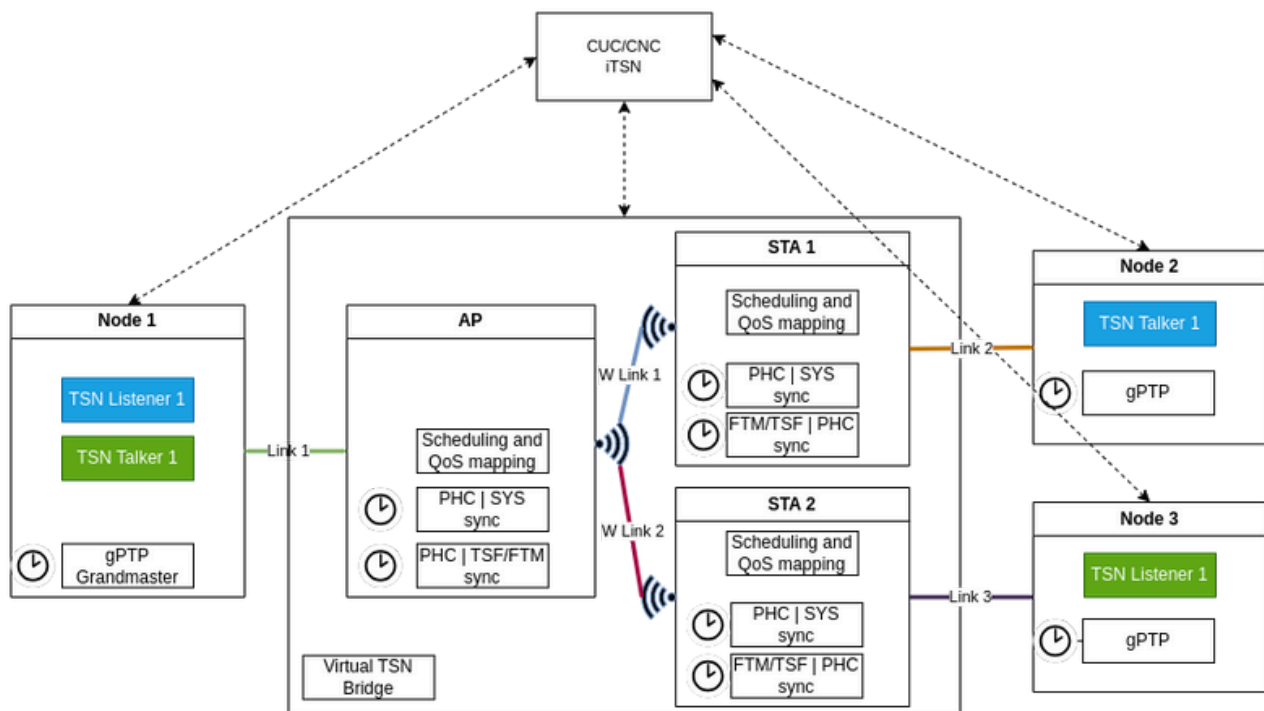
Figure 164: Reference architecture for OWTSN.
