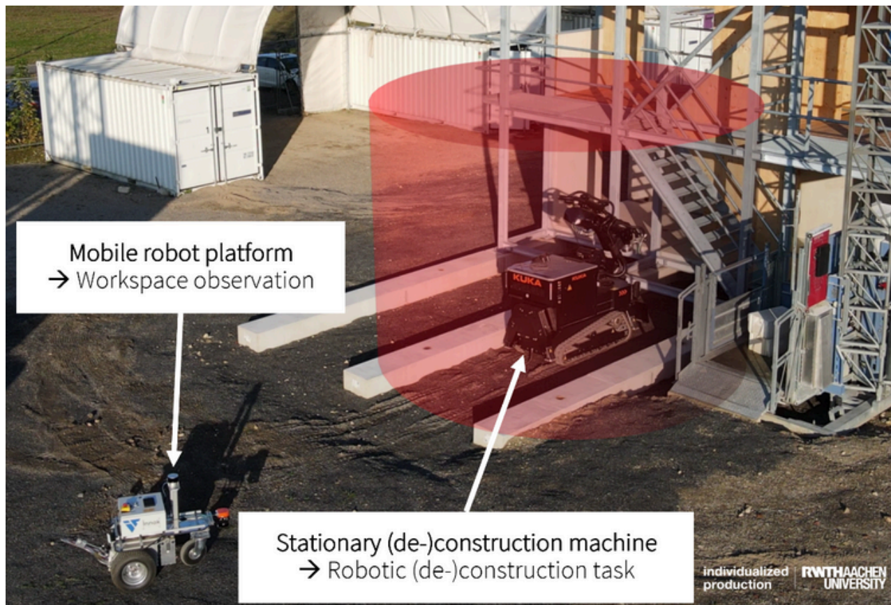
Figure 36: Overall deconstruction setup on the Reference Construction Site, Aachen https://doi.org/10.5281/zenodo.14755973
