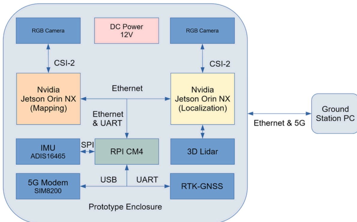
Hardware Diagram of VINS-RTK-Mapper
