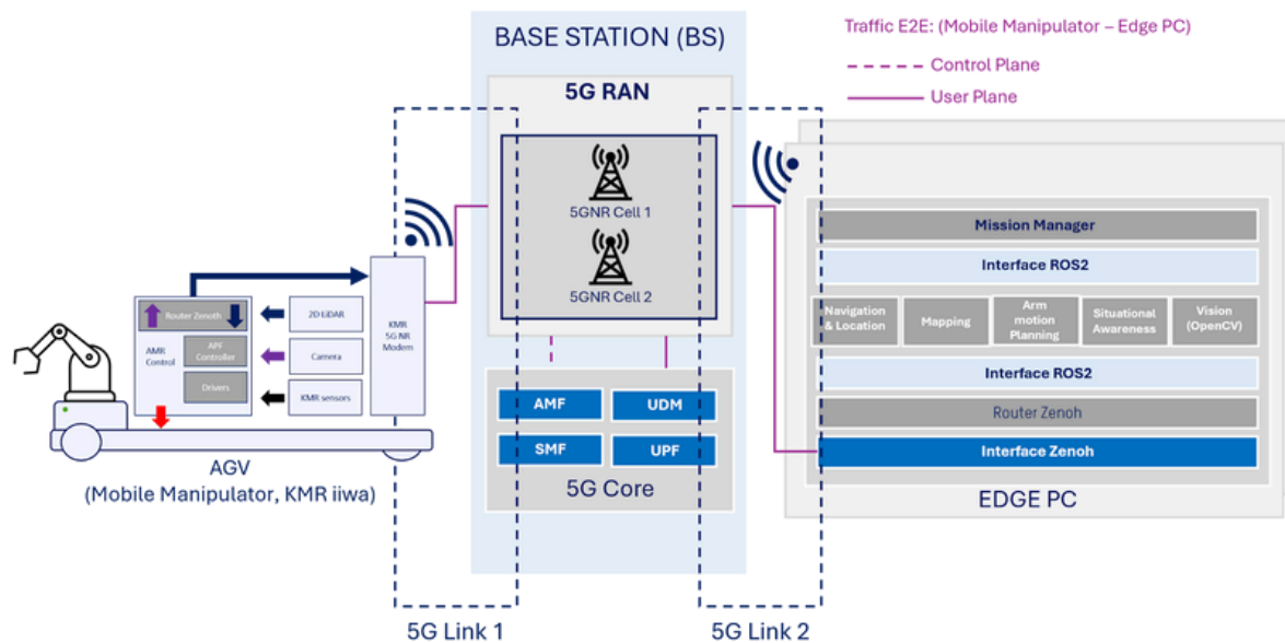
Figure 106: MM-IA: Function architecture of 5G communications
