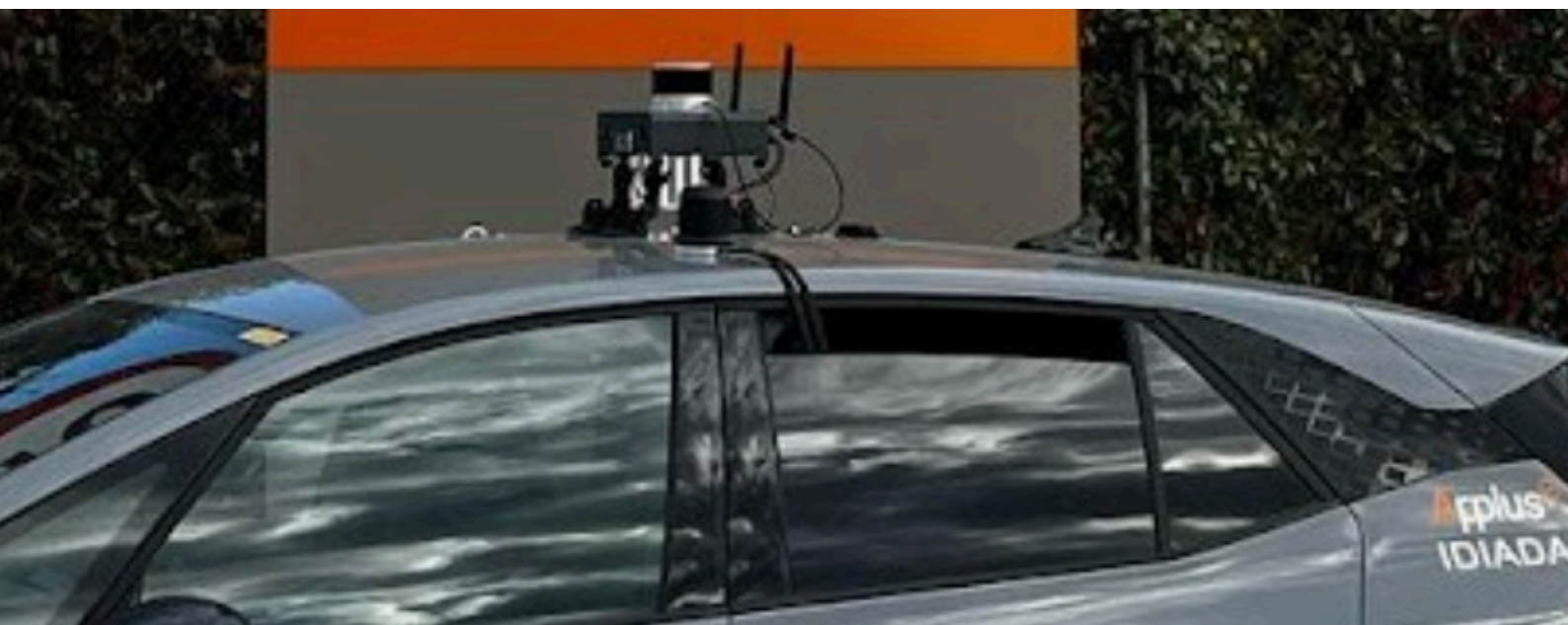
Figure 149: Prototype attached to Test Vehicle
