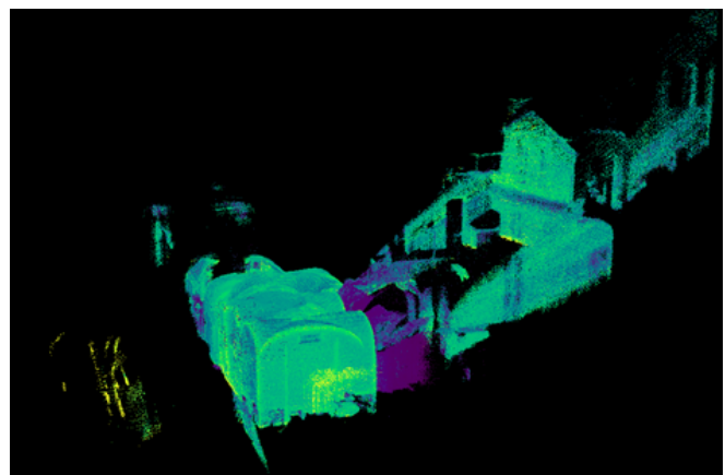
Figure 89: left - robot fully equipped (arm, lidar, mini-computer, 5G Modem); right: map of the full scene
