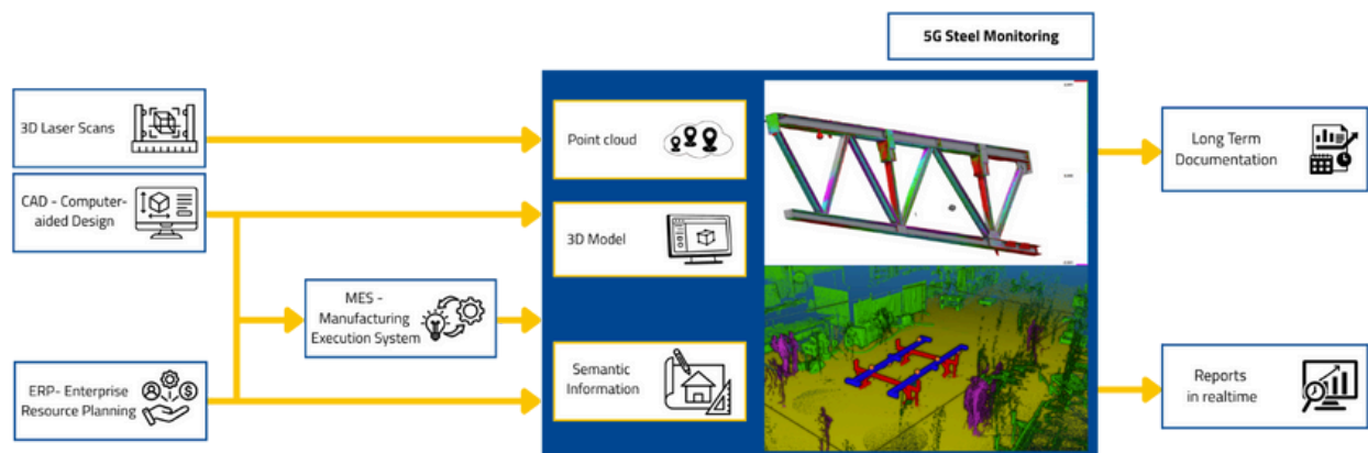
Figure 118: Integration of 5G Steel Monitoring
