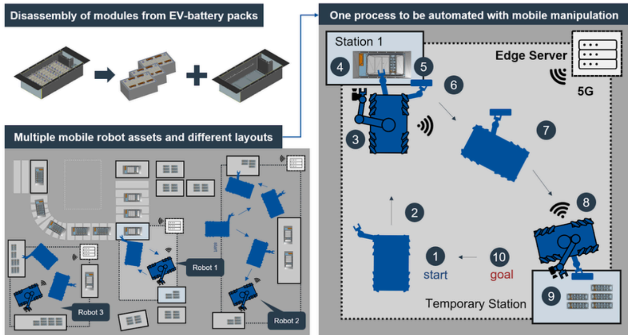
Figure 11: Edge-controlled automation with mobile manipulation for the disassembly of battery modules from EV-battery packs. Multiple robots for multiple assembly process (bottom left), process steps to be automated (right).
