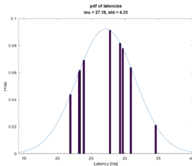
Figure 159: Latency experiments done in Spain (5G)
