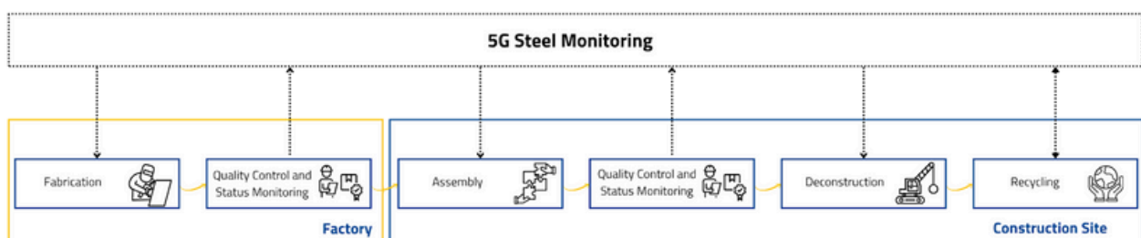
Figure 119: Processing in 5G Steel Monitoring
