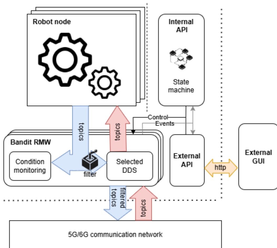
Figure 125: ROS2-BANDIT Architecture.
