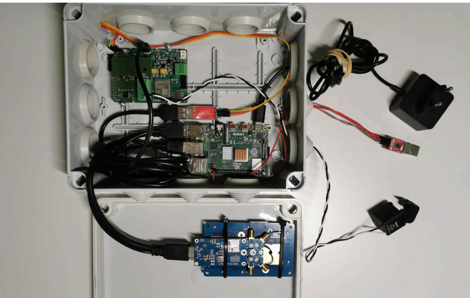
Figure 61: LENSE Trial Setup
