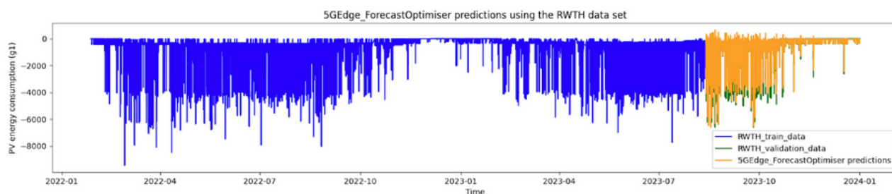
Figure 51: Behaviour of 5GEdge_ForecastOptimiser with respect to the RWTH data set.
