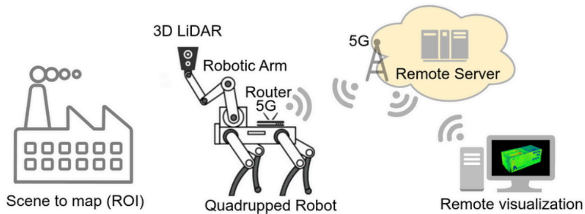
Figure 88: MARS schematic architecture of the robot, remote server and remote client
