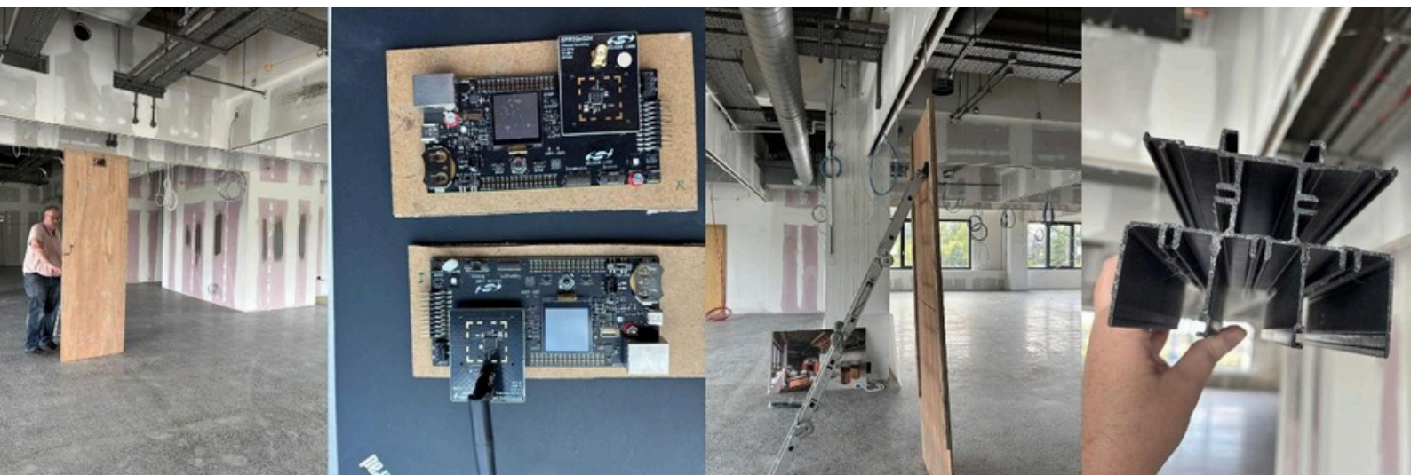
Figure 194: IntelliMat trial at HPBA showing Bluetooth 6 devices deployed in SmartGrid ceiling setup for real-time tracking and 5G integration
