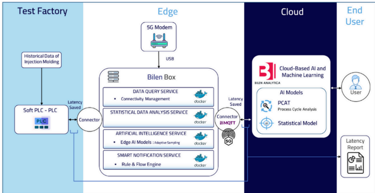
Figure 71: BILEN-5G High Level Architecture
