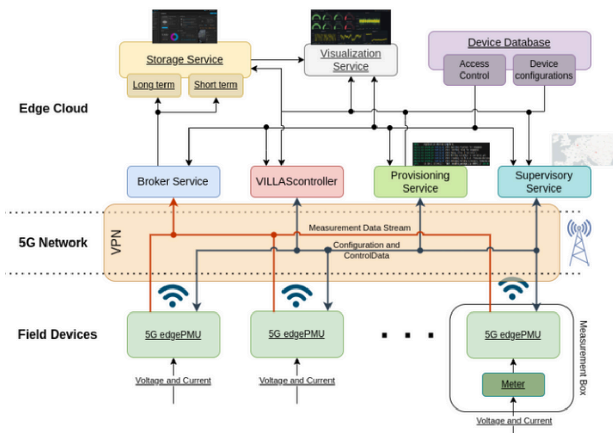
Figure 177: General architecture of the edge cloud and field side for the energy vertical
