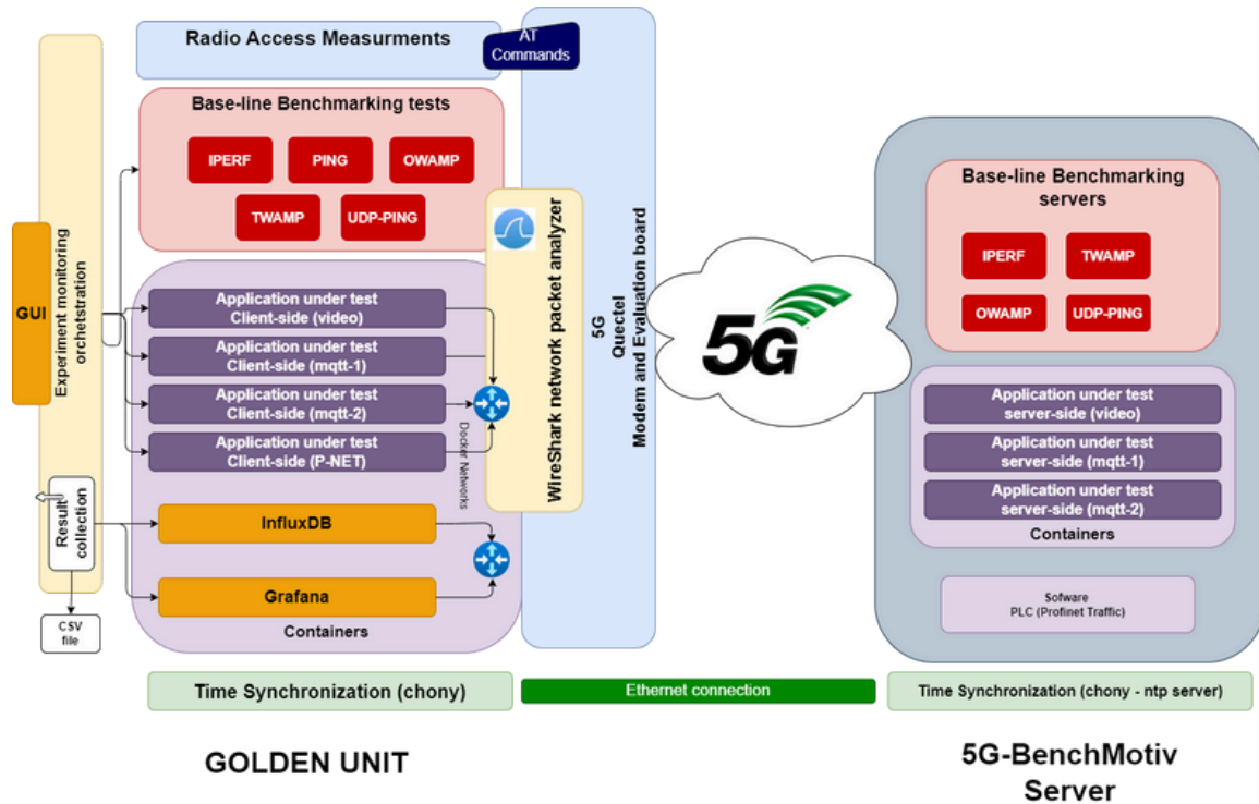
Figure 78: System deployment at Fraunhofer IPT premises.
