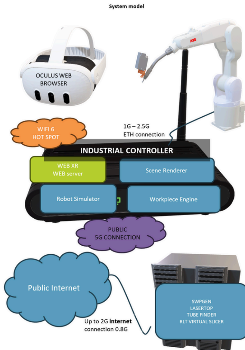
Figure 64: General scheme of the system
