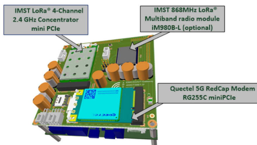
Figure 101: Extension Board design
