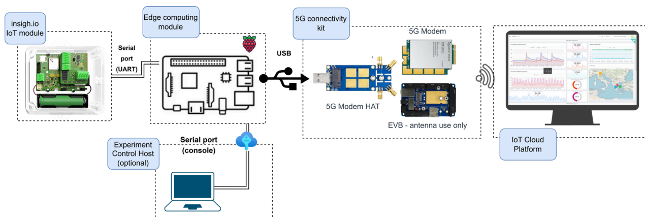
Figure 60: LENSE 5G-IoT Minimum Viable Product Architecture
