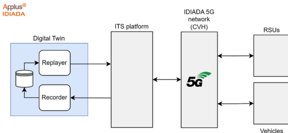
Figure 20: Architecture for replay functionality.
