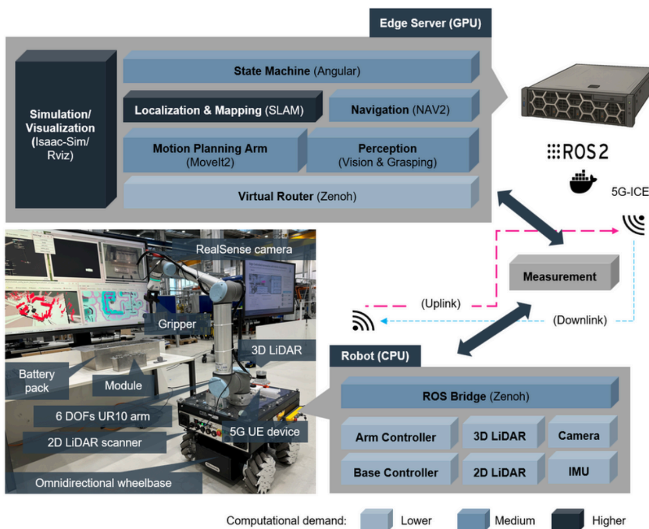
Figure 12: Hardware and ROS 2-based software architecture of the edge-controlled mobile automation use case. Hardware components of the robot are shown in the bottom left; edge and onboard software components are color-coded by computational demand. Monitoring pipeline is also illustrated.
