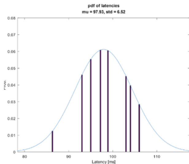
Figure 158: Latency experiments done in Turkey (LTE network)
