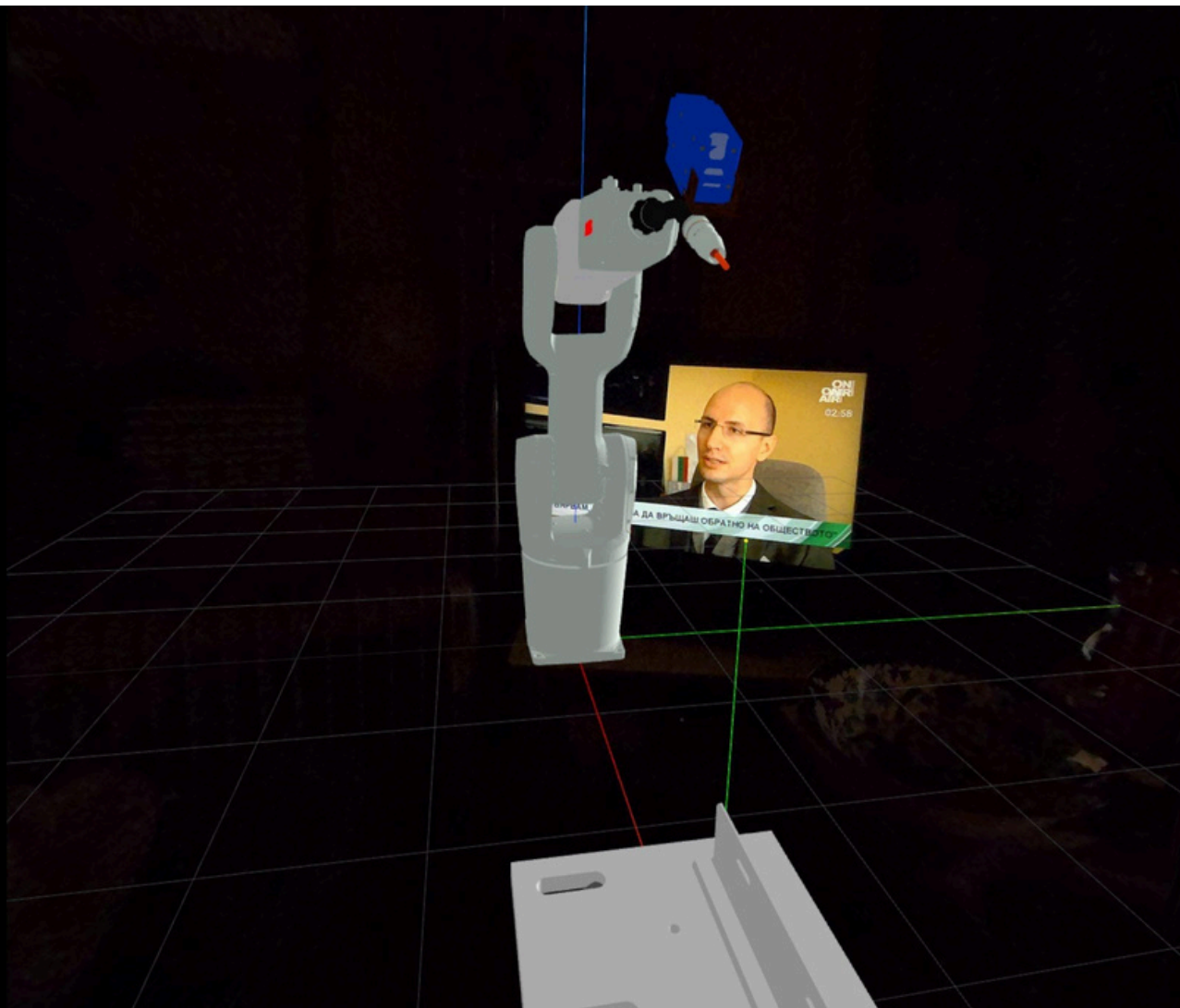
Figure 66: XR Glasses provide visualisation of proposed welding path including seam tracker simulation
