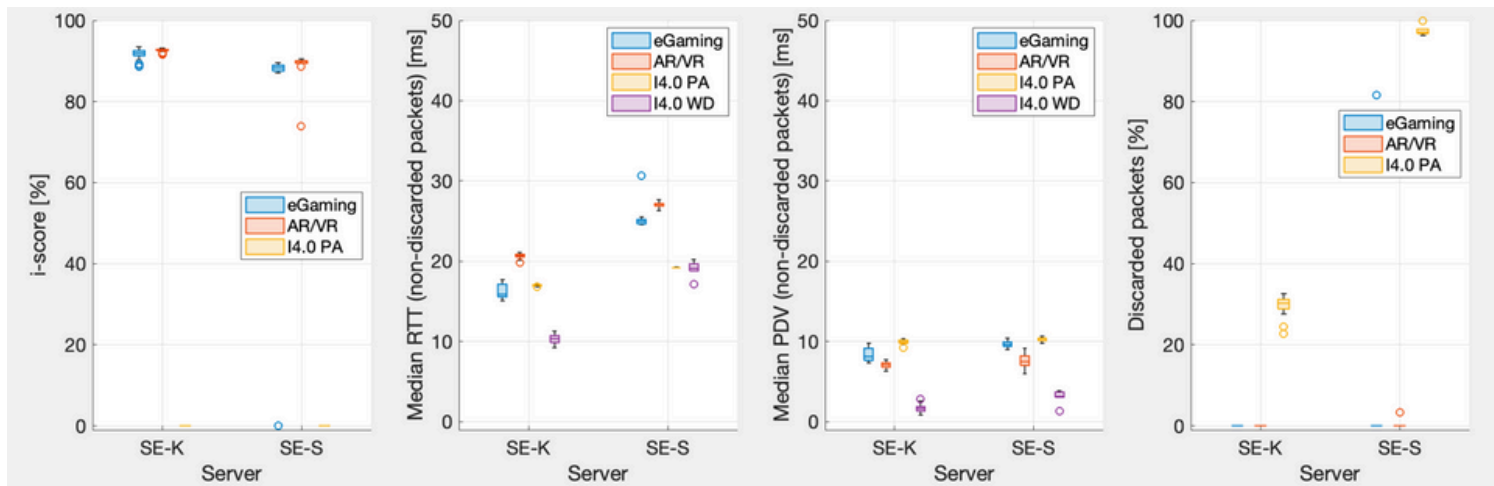
Figure 142: QoS/QoE performance obtained in the CARL-W testbed during the ITU-T interactivity tests, for different traffic patterns and server locations. QoS/QoE metrics: interactivity score (i-score [%]), packet round trip time (RTT [ms]), packet delay variation (PDV [ms]), and discarded packets [%]. Traffic Patterns: eGaming, AR/VR, I4.0 Process Automation (PA), and Industry 4.0 Watchdog (WD); Server location: edge (SE-K) vs. cloud (SE-S).
