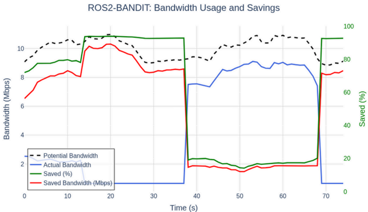
Figure 127: Traffic saving during a pick-and-place task.
