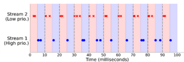
Figure 168: Tx timeline with scheduling.
