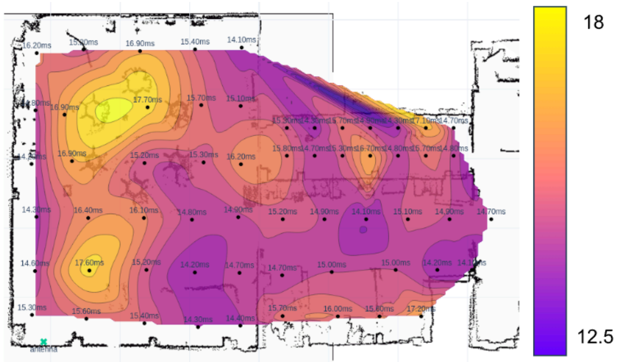
Figure 98: Example QoS heatmap. Delay of a private 5G network, in ms
