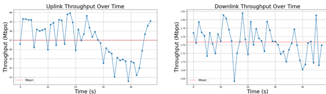
Figure 15: Uplink (left) and Downlink (right) throughput over time during Trial 9 of the A-B-A navigation task.
