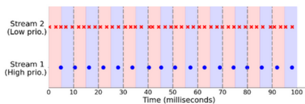
Figure 167: Tx timeline without scheduling.
