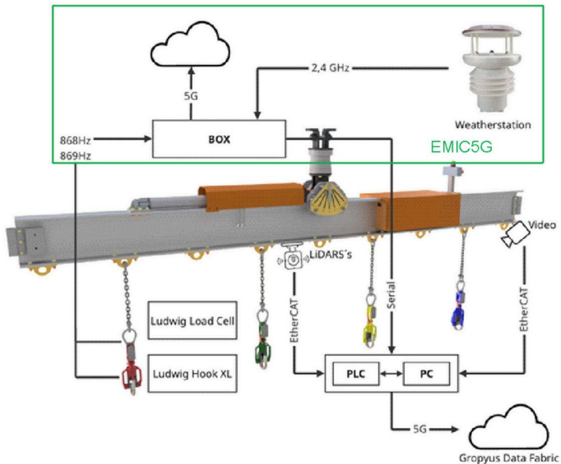
Figure 103: FACT-5G functional diagram
