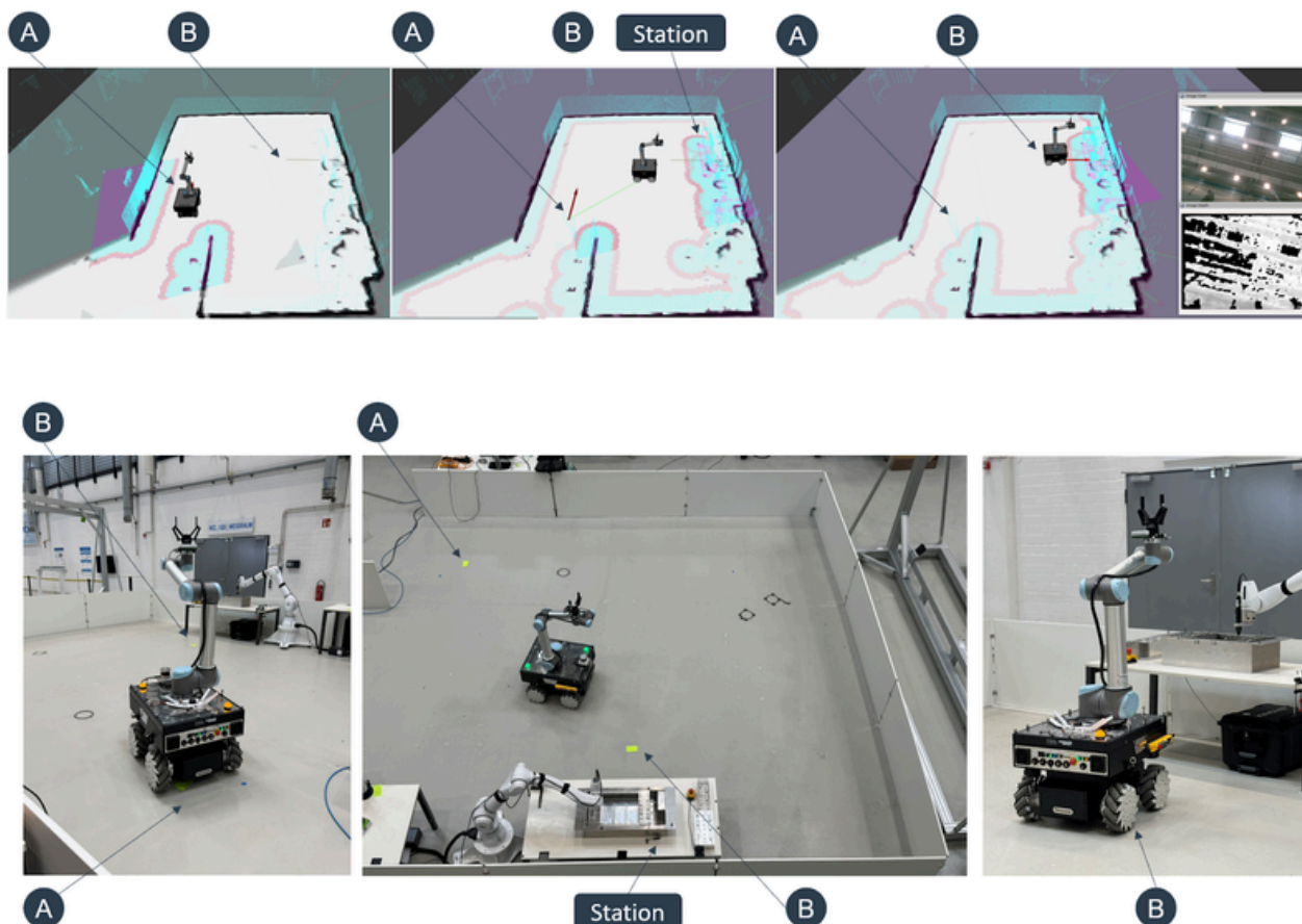
Figure 13: Edge-executed software stack for cloud-based localization and navigation (top). Operator-defined positions A and B are configured via the GUI interface. Photographs of the A-B-A navigation trials conducted at the WZL Testbed (bottom).
