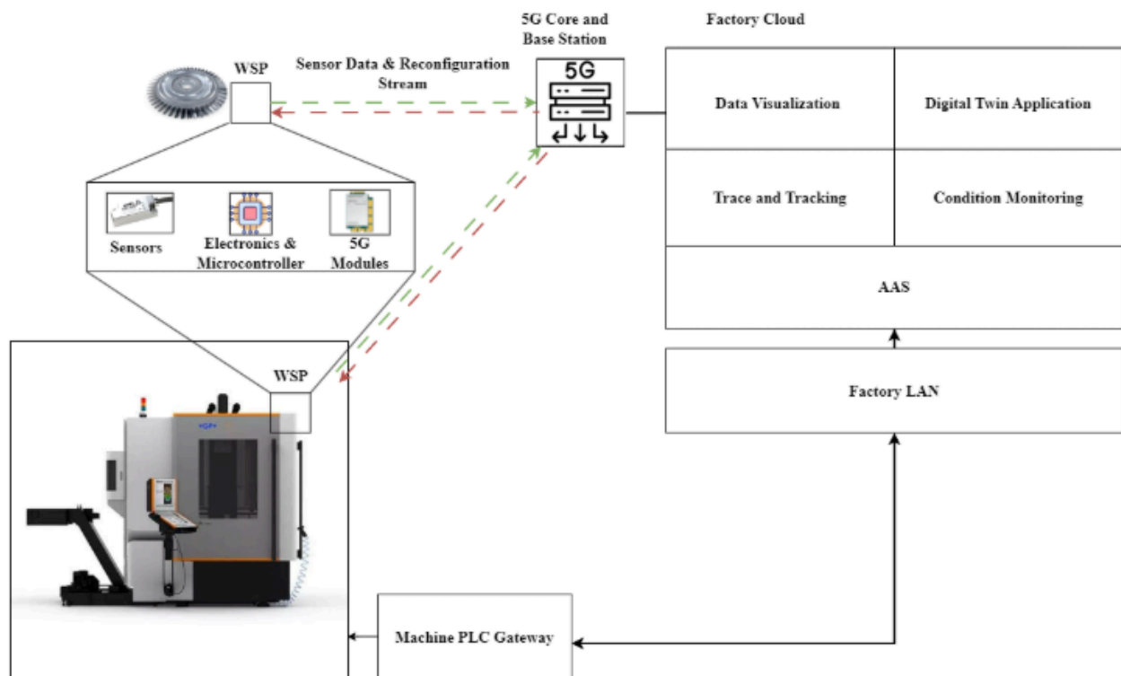
Figure 6: Architecture of the wireless sensor platform.
