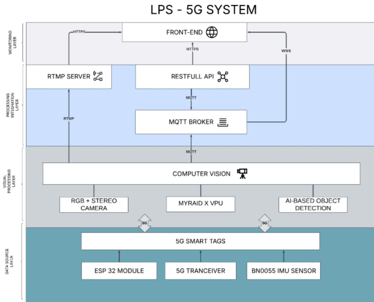
Figure 186: LPS-5G system Architecture
